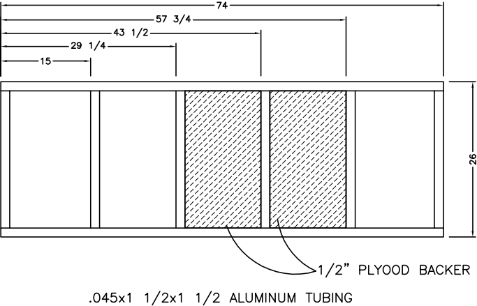
BUNK FRAME TOP VIEW
