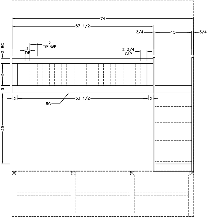
RAIL AND LADDER (HARDWOOD)
