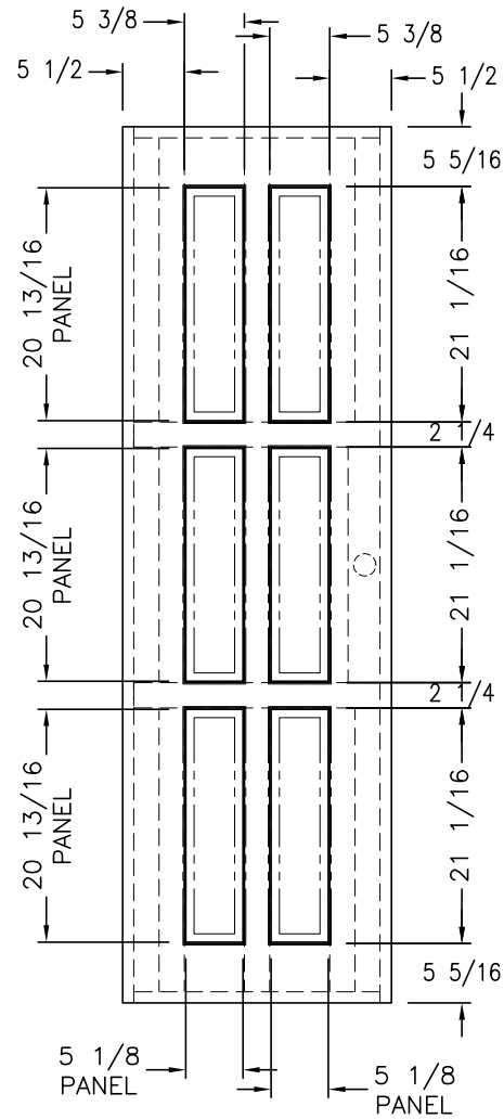
DOOR ROUTING
