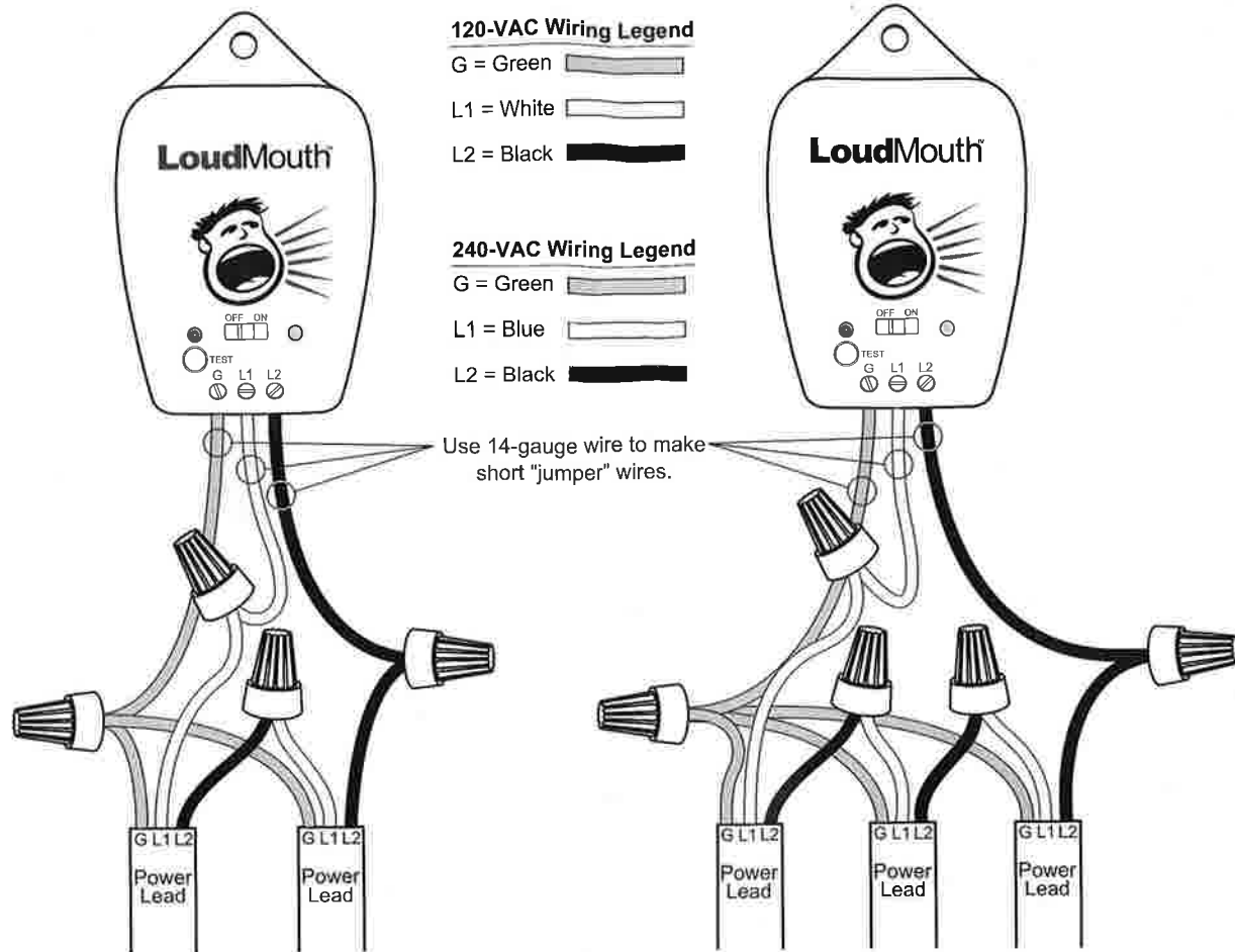
Schematic showing how to connect three heating mats or cables to the LoudMouth for monitoring during installation.
