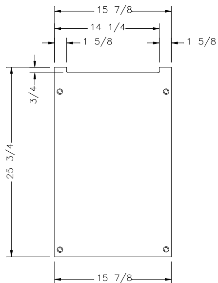
CABINET FRONT COVER 3.6mm LUAN VINYL WRAPPED
