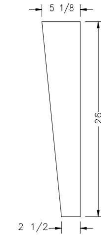
PANEL, RIGHT & LEFT
