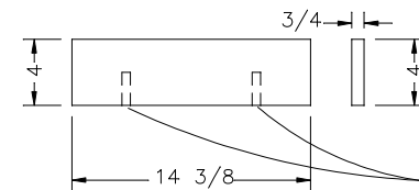
FRONT BOTTOM
