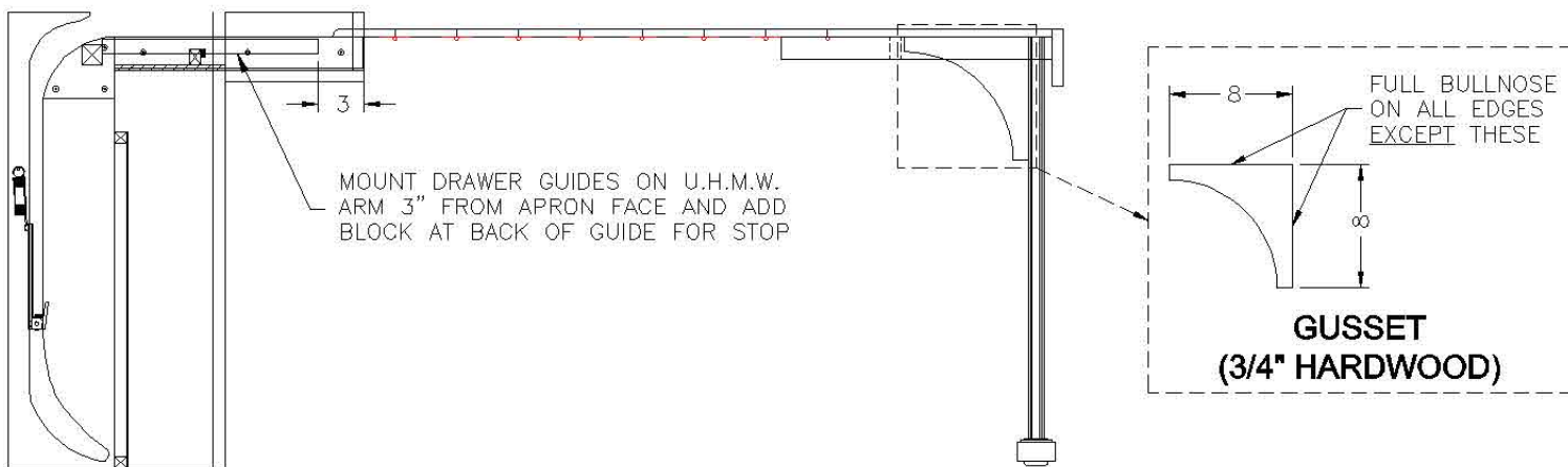
ROLL AWAY TABLE SIDE VIEW
