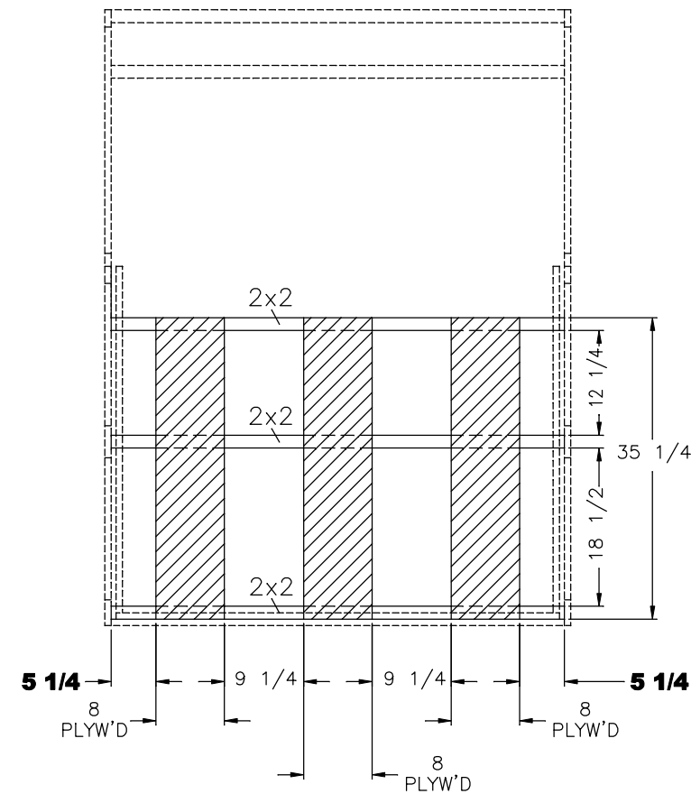
ROLLER BACKER 3/4 PLYWOOD (BOTTOM VIEW)
