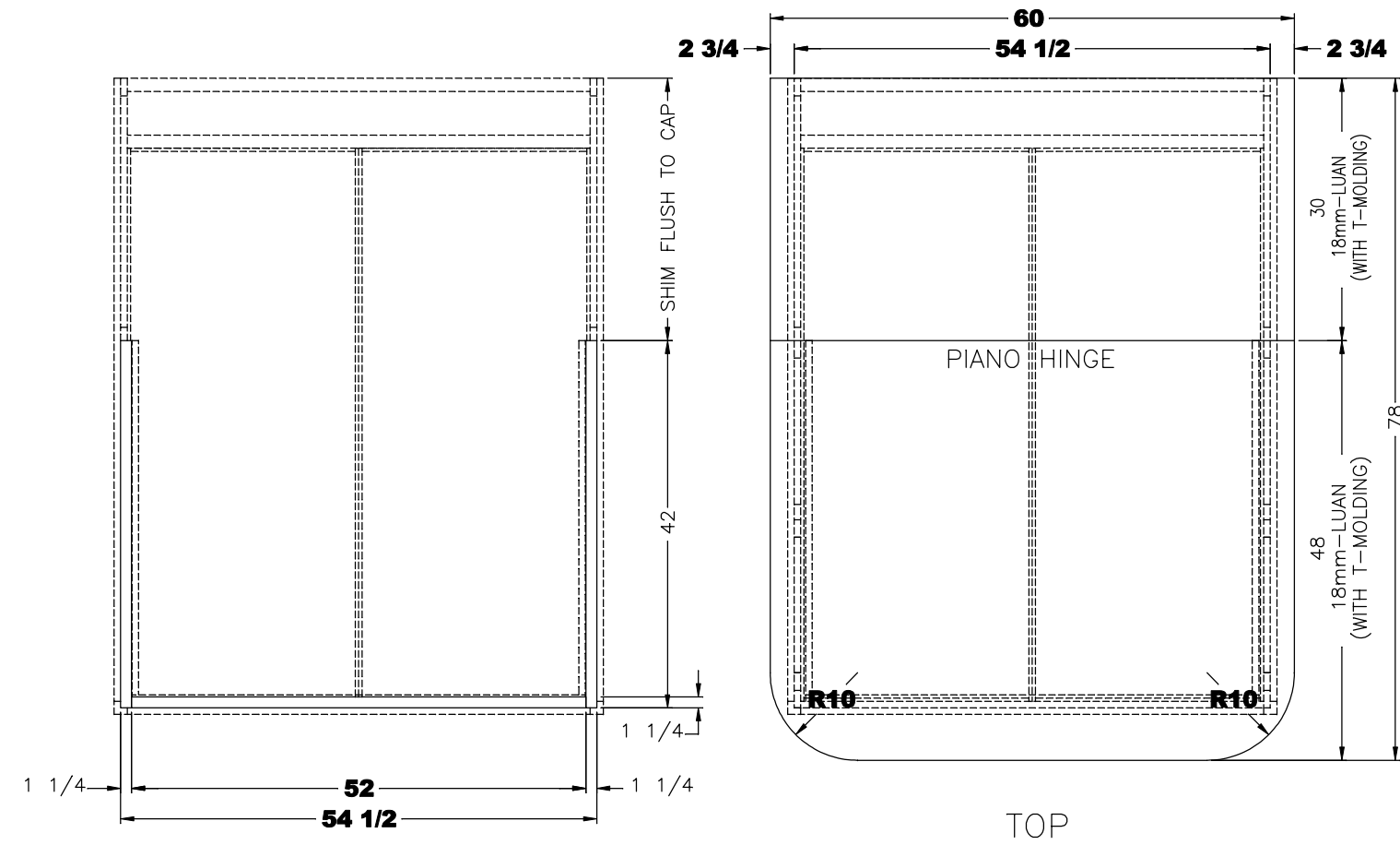
TOP CAP 3/4" FIBERCORE NOTE: FINISH ALL INTERIOR EDGES
