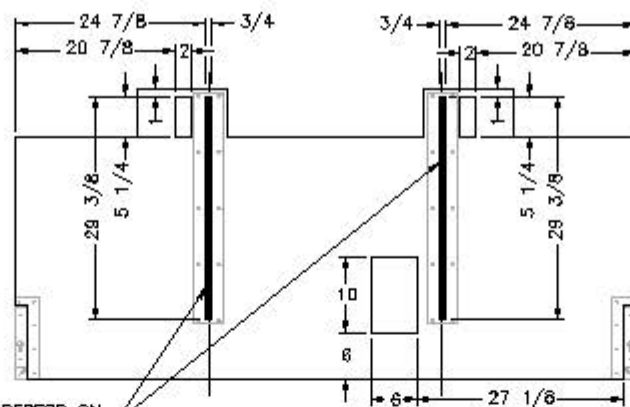
BOTTOM VIEW (HUBER)
