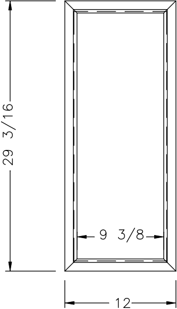
MIRROR FRAME SEE PROFILE 'A' FOR MOLDING
