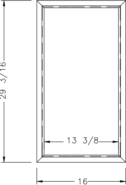
MIRROR FRAME SEE PROFILE 'A' FOR MOLDING
