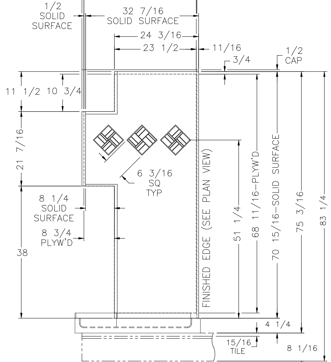
VIEW A
