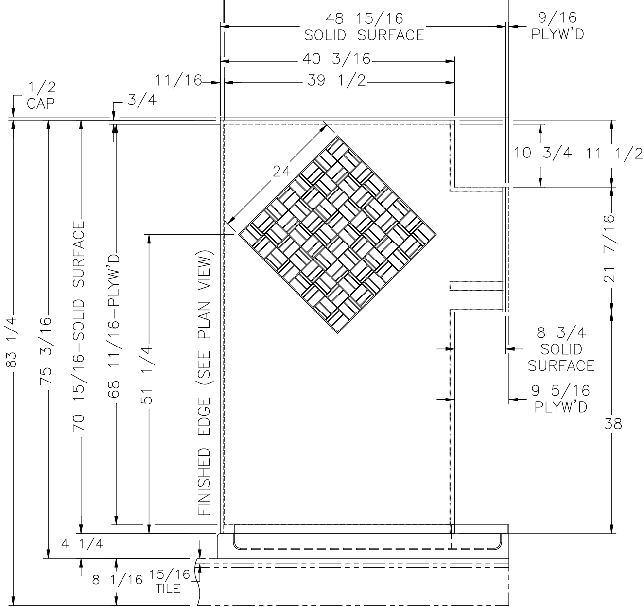
VIEW B
