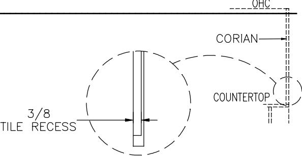
RECESS TILE VIEW (SCALE 4X) (T360)
