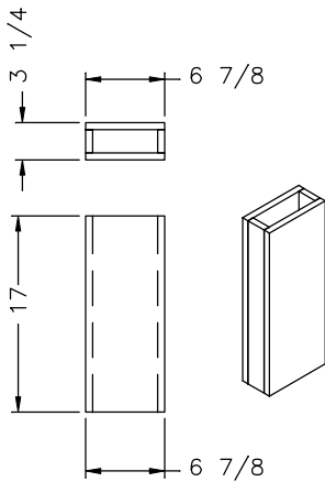
5/8 PLYWOOD BOX SPLASH BUILD UP
