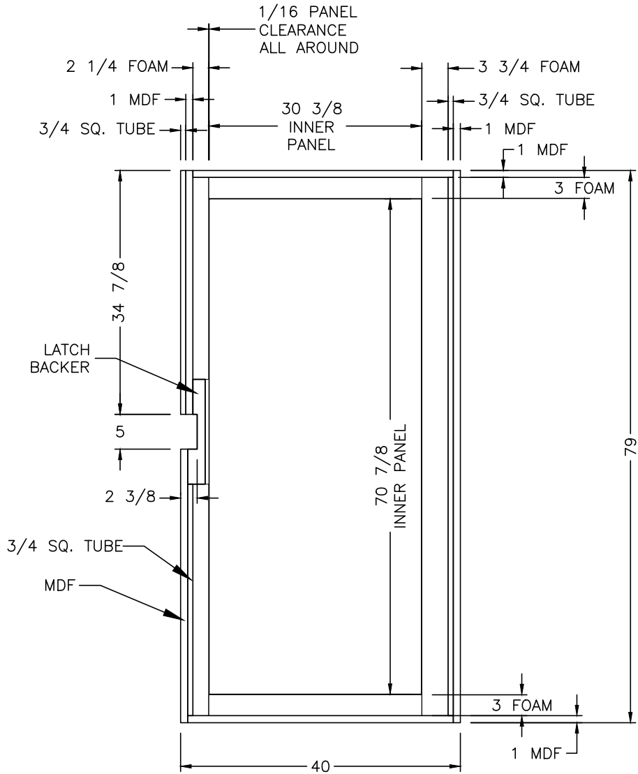
POCKET DOOR CONSTRUCTION
