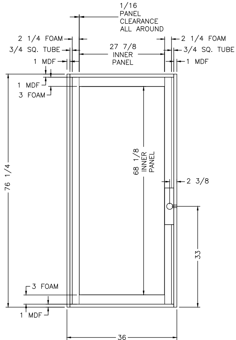
SWING DOOR CONSTRUCTION
