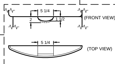
DRAWER CUT OUT DETAIL (LAF & RAF)
