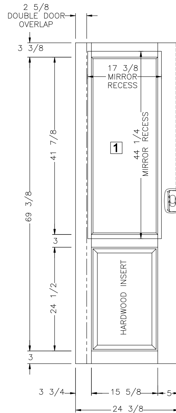
KITCHEN SIDE
