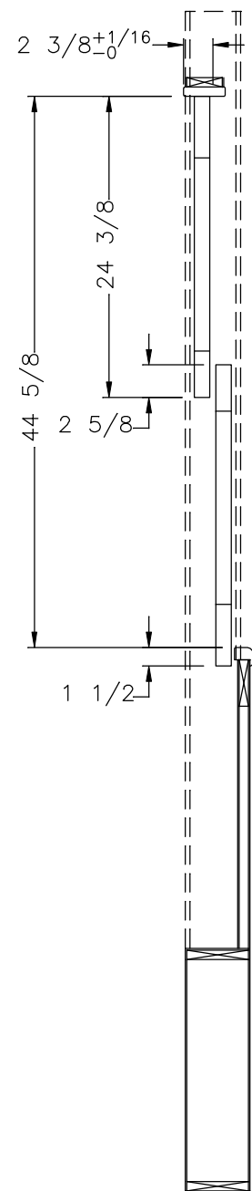
PLAN VIEW
