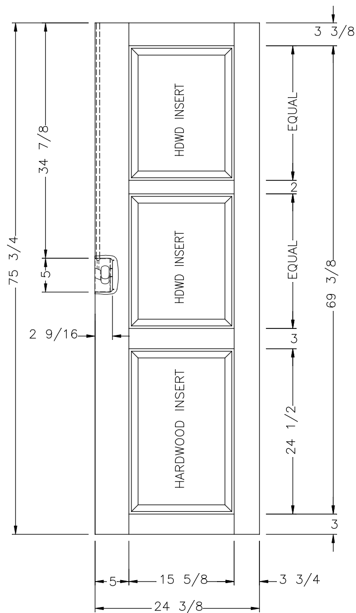
BEDROOM SIDE
