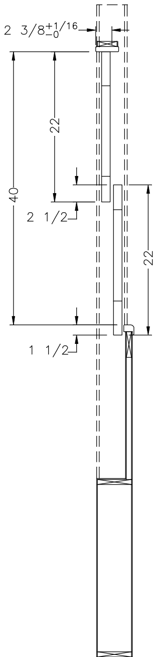
PLAN VIEW
