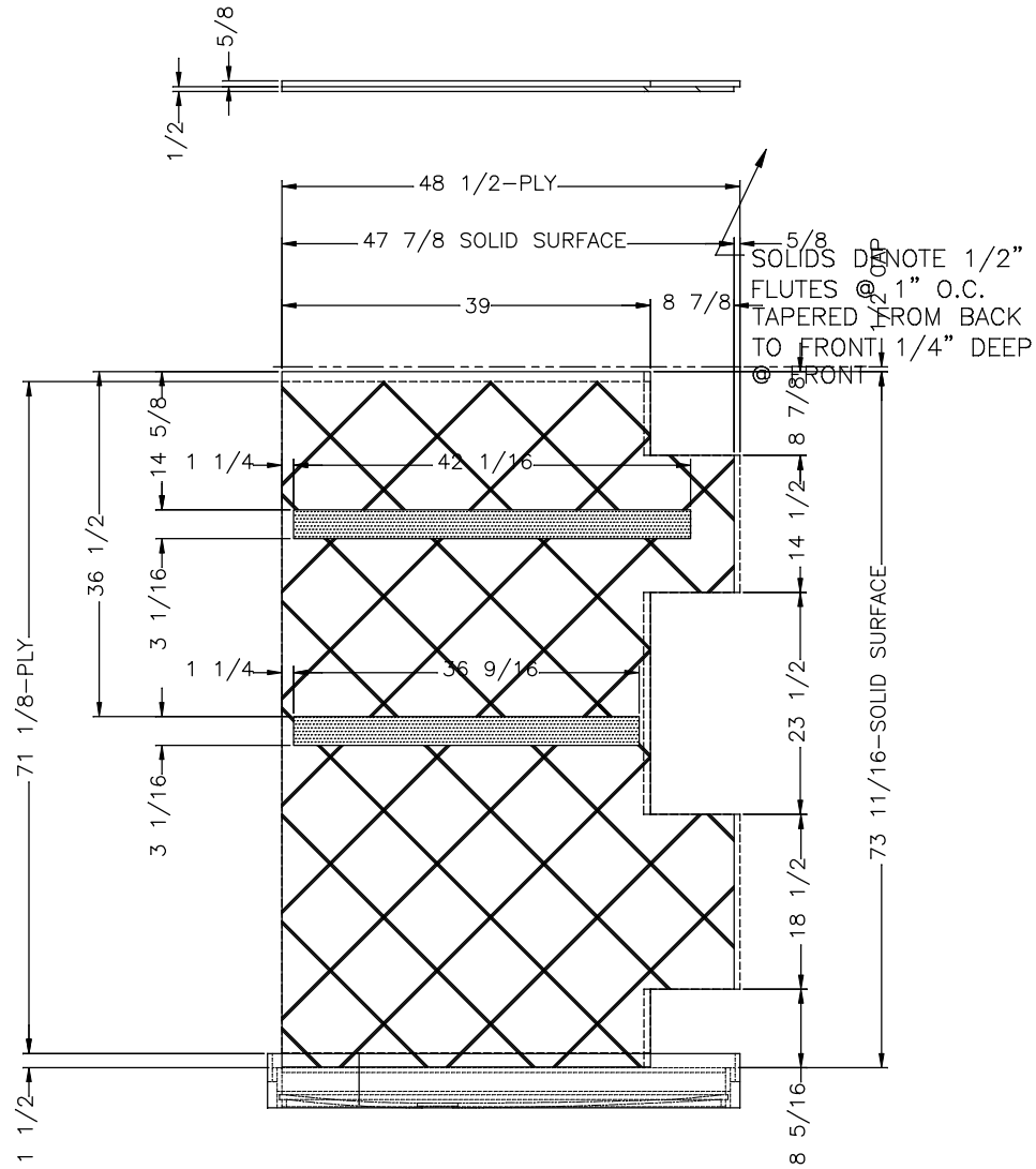
VIEW A
