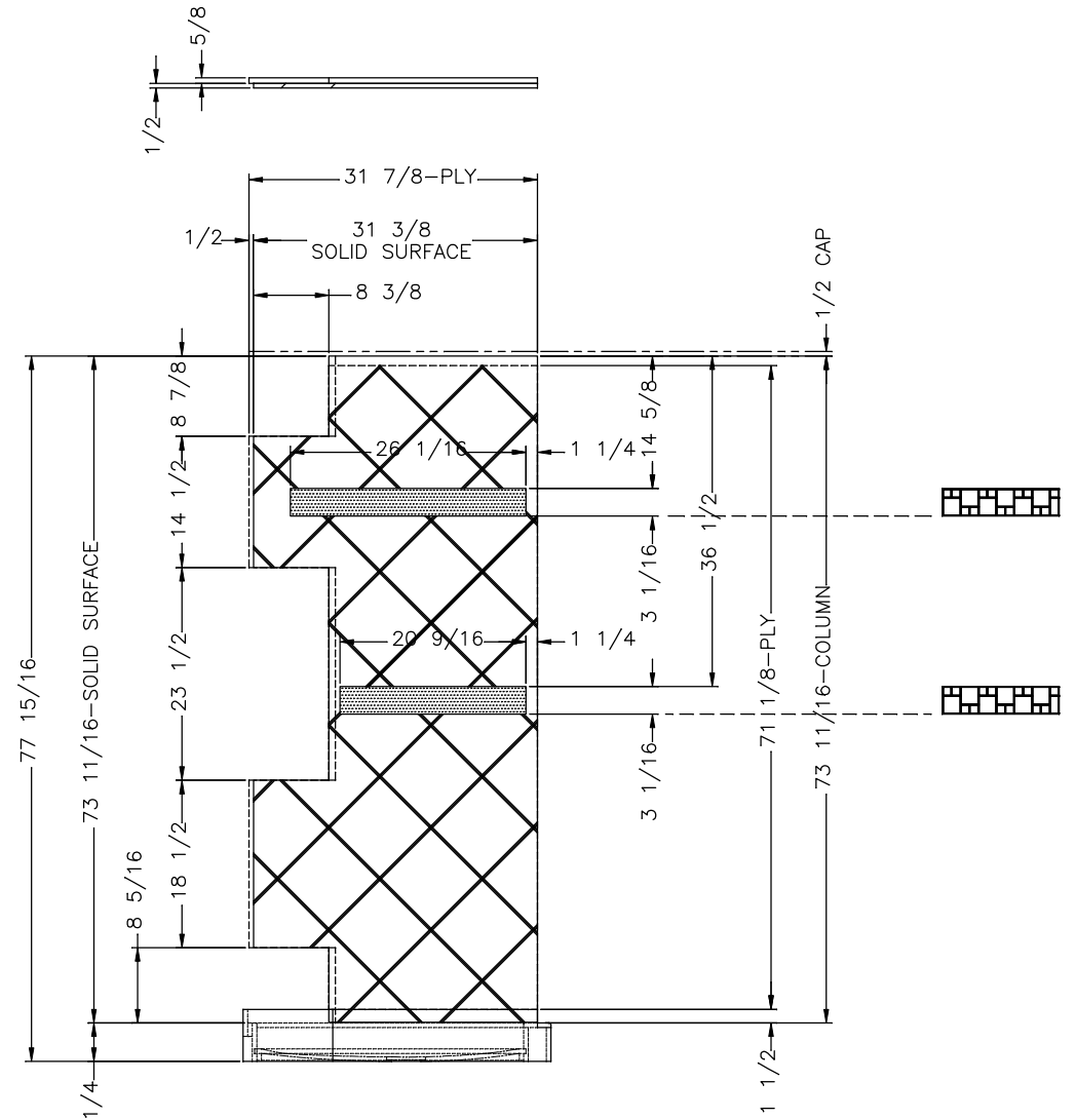
VIEW B
