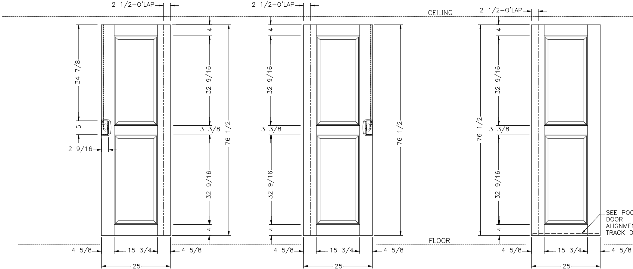
BEDROOM SIDE
