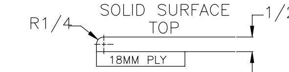
SECTION A (BACK EDGE ONLY) SCALE=4X (SEE COUNTERTOP EDGES PRINT FOR THE OTHER 3 EDGES)
