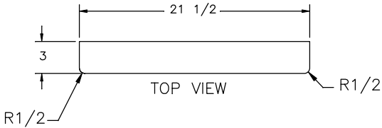
LEDGE DETAIL
