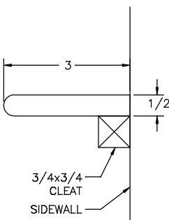
SIDE VIEW SCALE=4X
