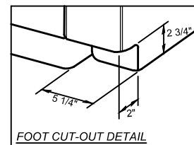
FOOT CUT-OUT DETAIL
