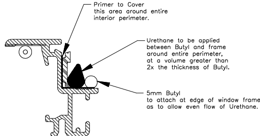
SCALE : FULL
