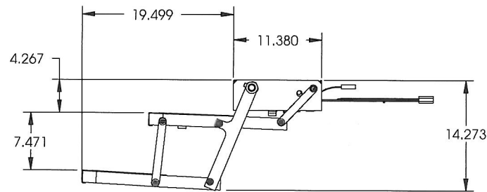
DIMENSIONS REFERENCE
