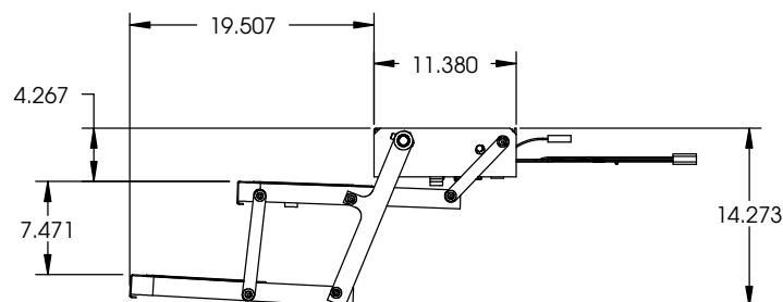
DIMENSIONS REFERENCE
