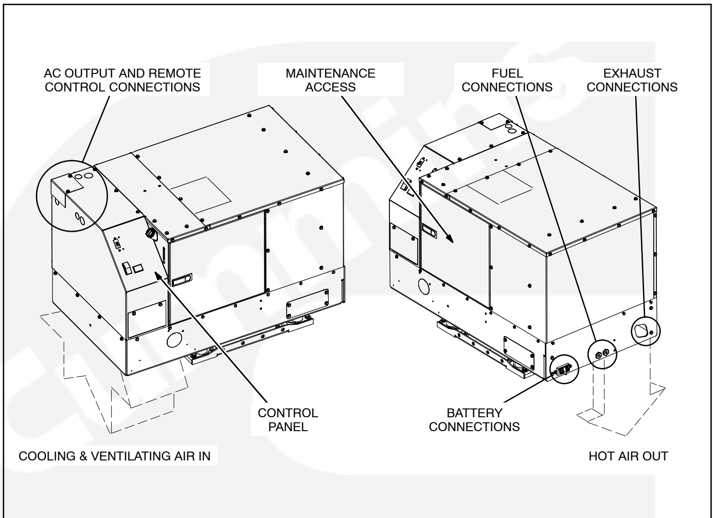
FIGURE 1-4. TYPICAL GENSET
