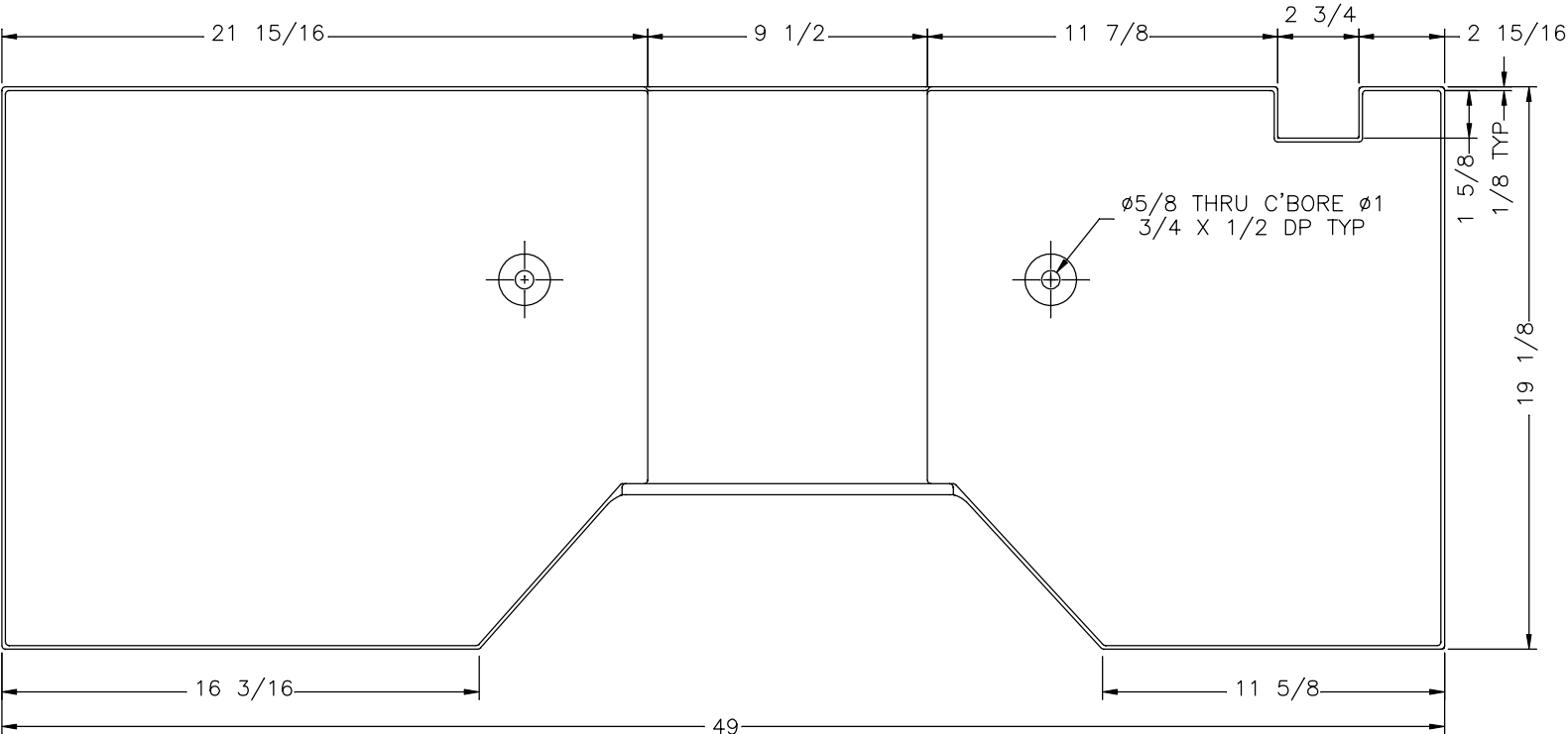
TOP VIEW
