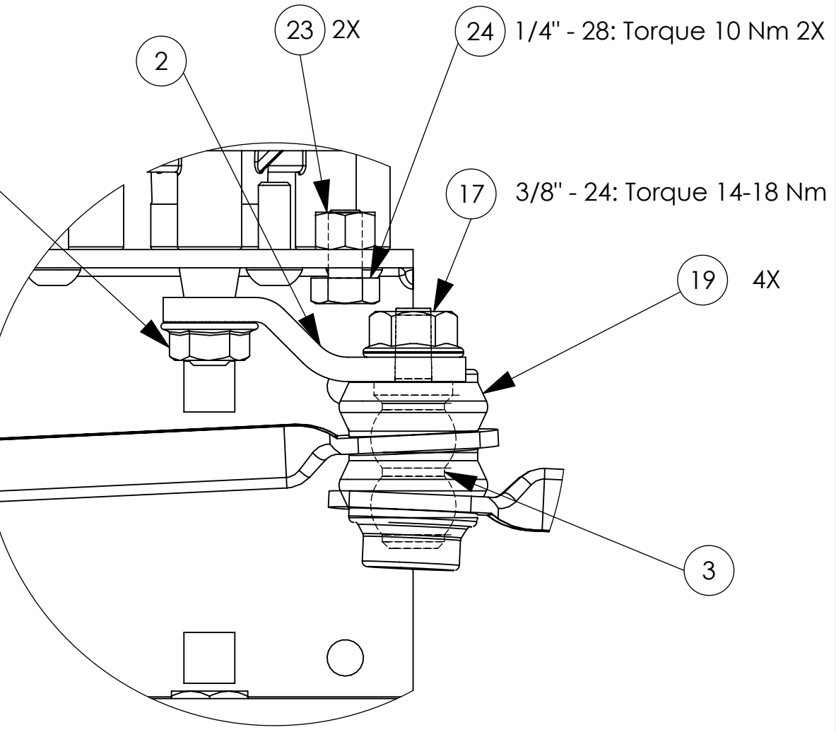
DETAIL C SCALE 1 : 1 Top view shown without brackets.
