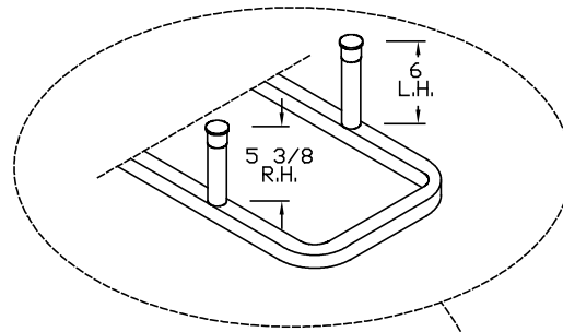
BOTTOM LEG DETAIL
