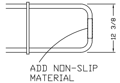
* REAR LADDER DETAIL
