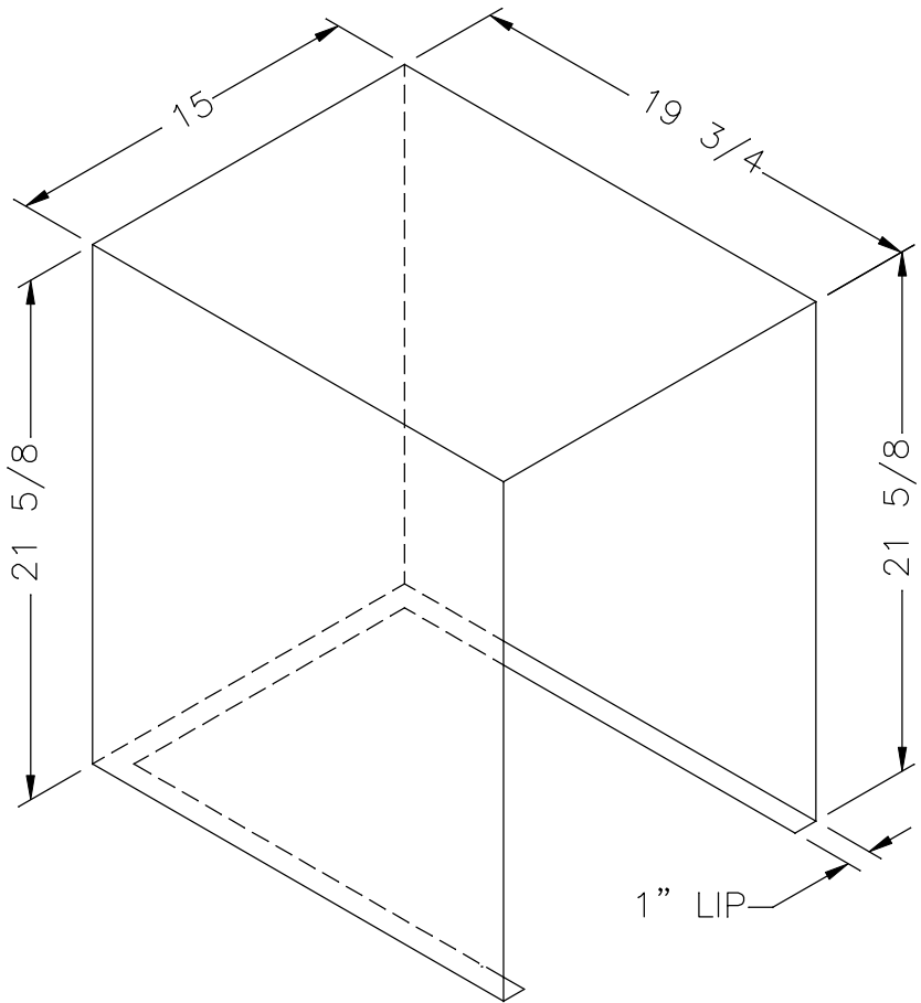
ISOMETRIC VIEW
