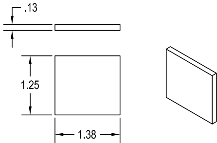
2 SWITCH TRIGGER PLATE SCALE 2X
