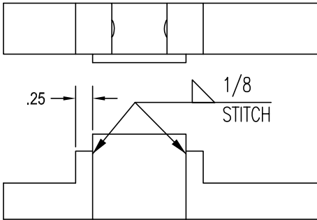
ACTUATOR SLIDE BLOCK WELDMENT
