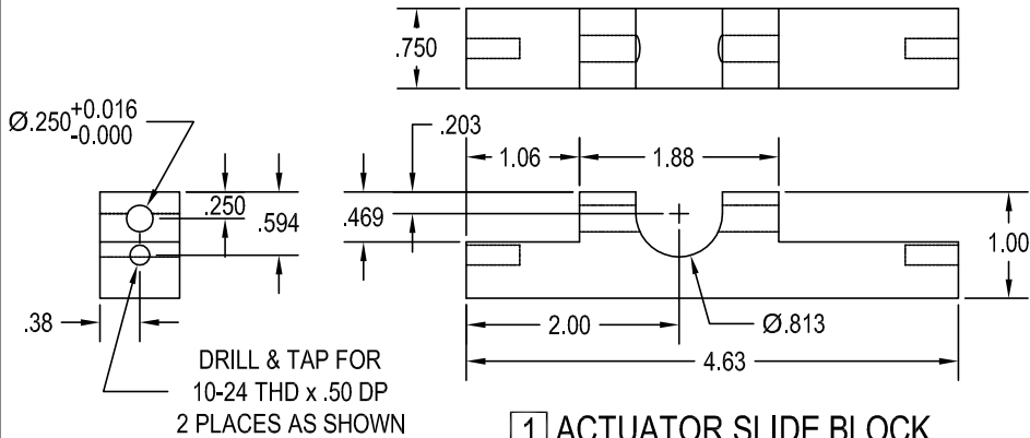
1 ACTUATOR SLIDE BLOCK SCALE 2X
