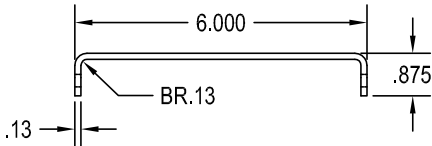
2 CLAMP PIVOT BRACKET
