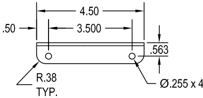
2 CLAMP PIVOT BRACKET
