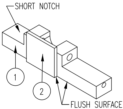
ACTUATOR SLIDE BLOCK WELDMENT
