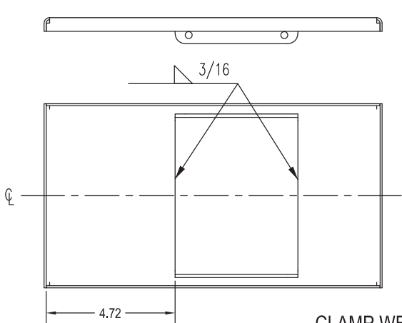
CLAMP WELDMENT
