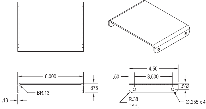
2 CLAMP PIVOT BRACKET
