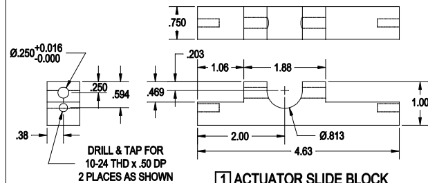
1 ACTUATOR SLIDE BLOCK SCALE 2X
