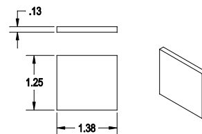
2 SWITCH TRIGGER PLATE SCALE 2X
