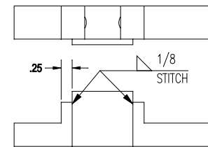
ACTUATOR SLIDE BLOCK WELDMENT
