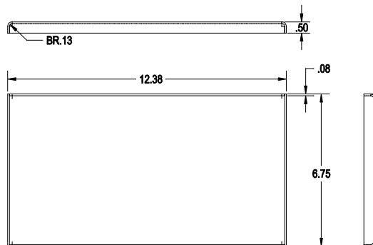
1 CLAMP
