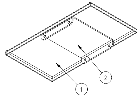
CLAMP WELDMENT
