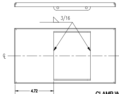
CLAMP WELDMENT
