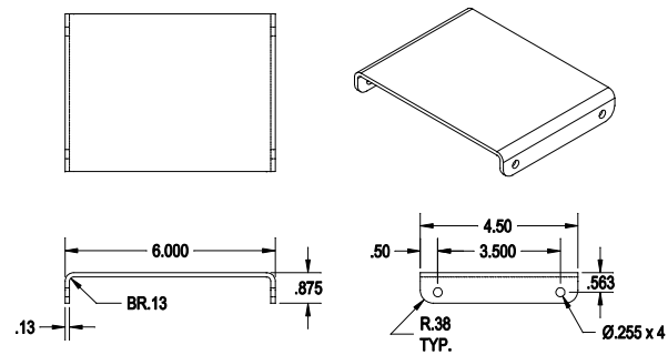
2 CLAMP PIVOT BRACKET
