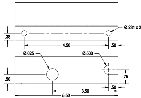
3 SWITCH COVER SCALE 2X
