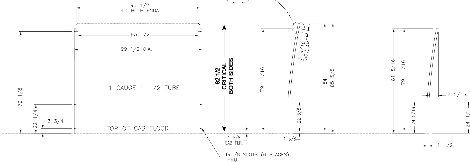
FRONT VIEW (TUBE BENT) WINDSHIELD REINFORCEMENT
