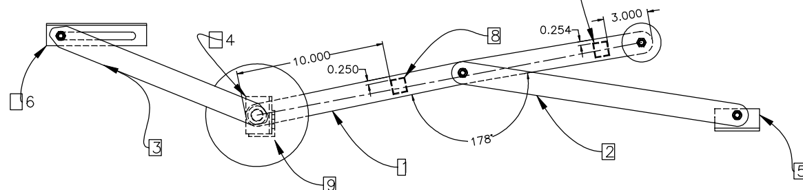
BED LIFT ASSEMBLY—SIDE VIEW
