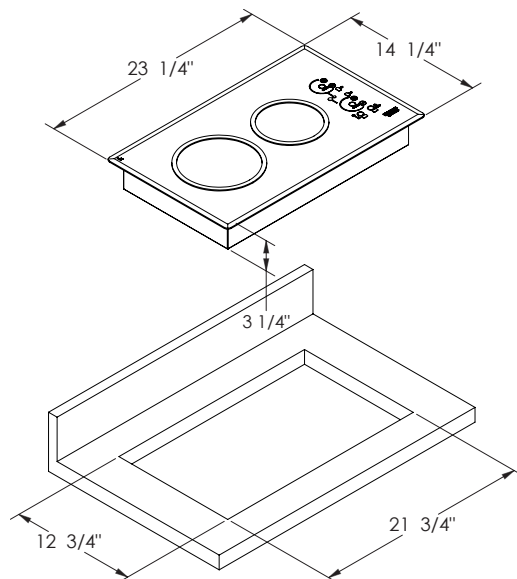
COUNTERTOP CUTOUT DIMENSIONS B41540L, B41549L, and B41541L
