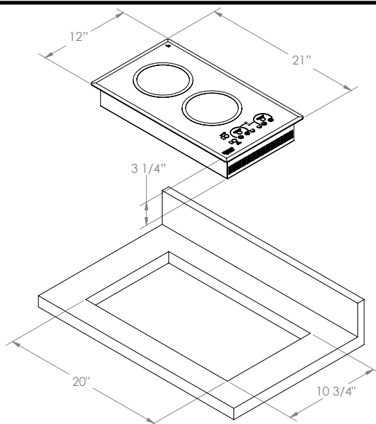
COUNTERTOP CUTOUT DIMENSIONS B41575L, B41579L, and B41576L
