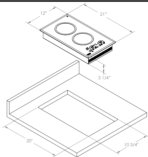
COUNTERTOP CUTOUT DIMENSIONS B41575, B41579, and B41576
