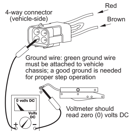
FIGURE 17: Connector
