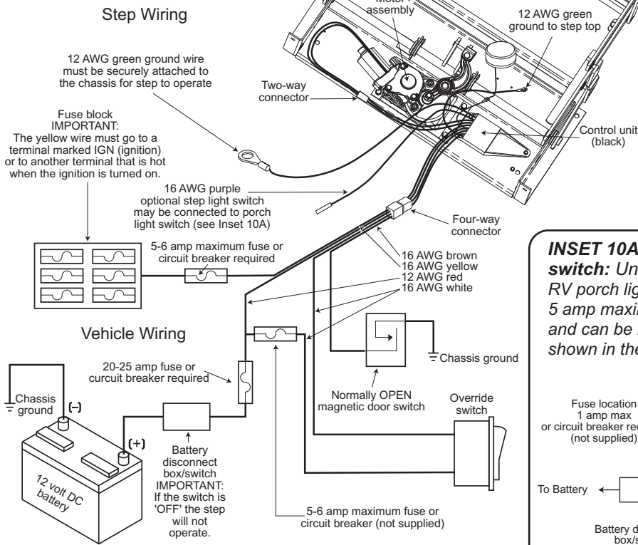
FIGURE 11: Wiring diagram for steps with door switch only operation
