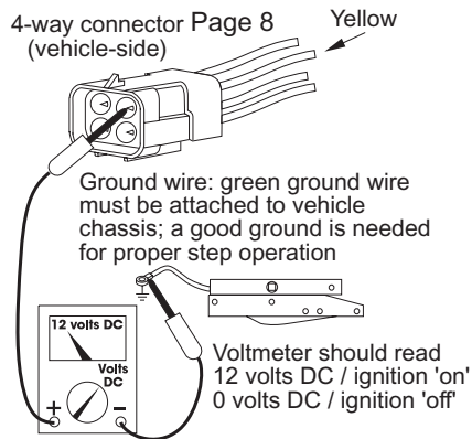
FIGURE 16: Ignition override
