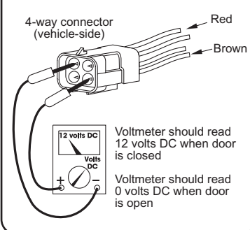
FIGURE 15: Door switch
