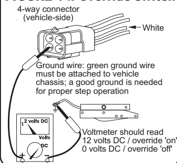
FIGURE 14: Override switch
