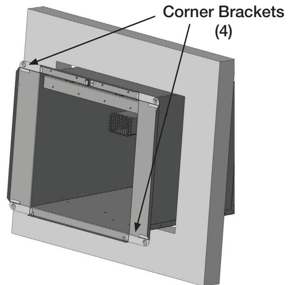
Installation in standard 6 gallon water heater opening with Standard Door Kit
