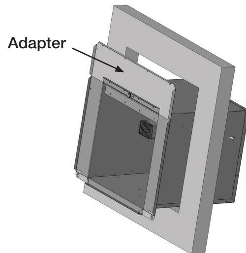
Installation in standard 10 gallon water heater opening with Large Door Adapter Kit
