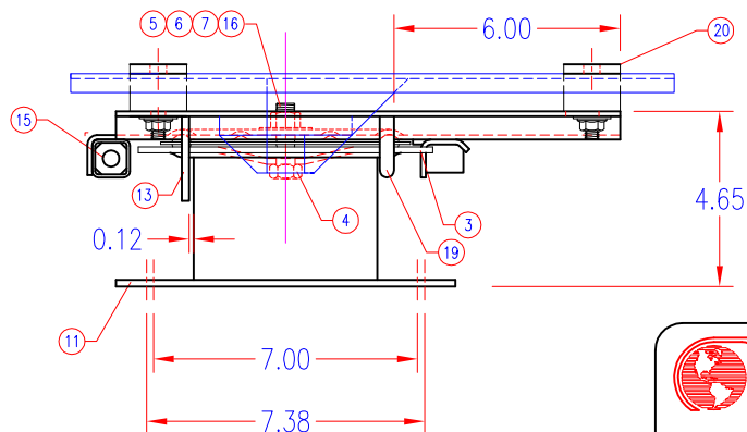
RH SIDE VIEW
