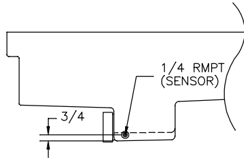
SENSOR LOCATION - VIEW C
