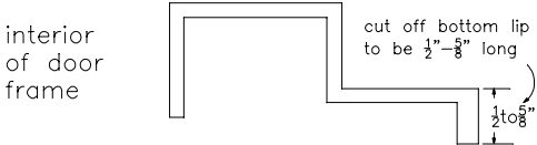
Enlarged View of bottom lip of door frame
