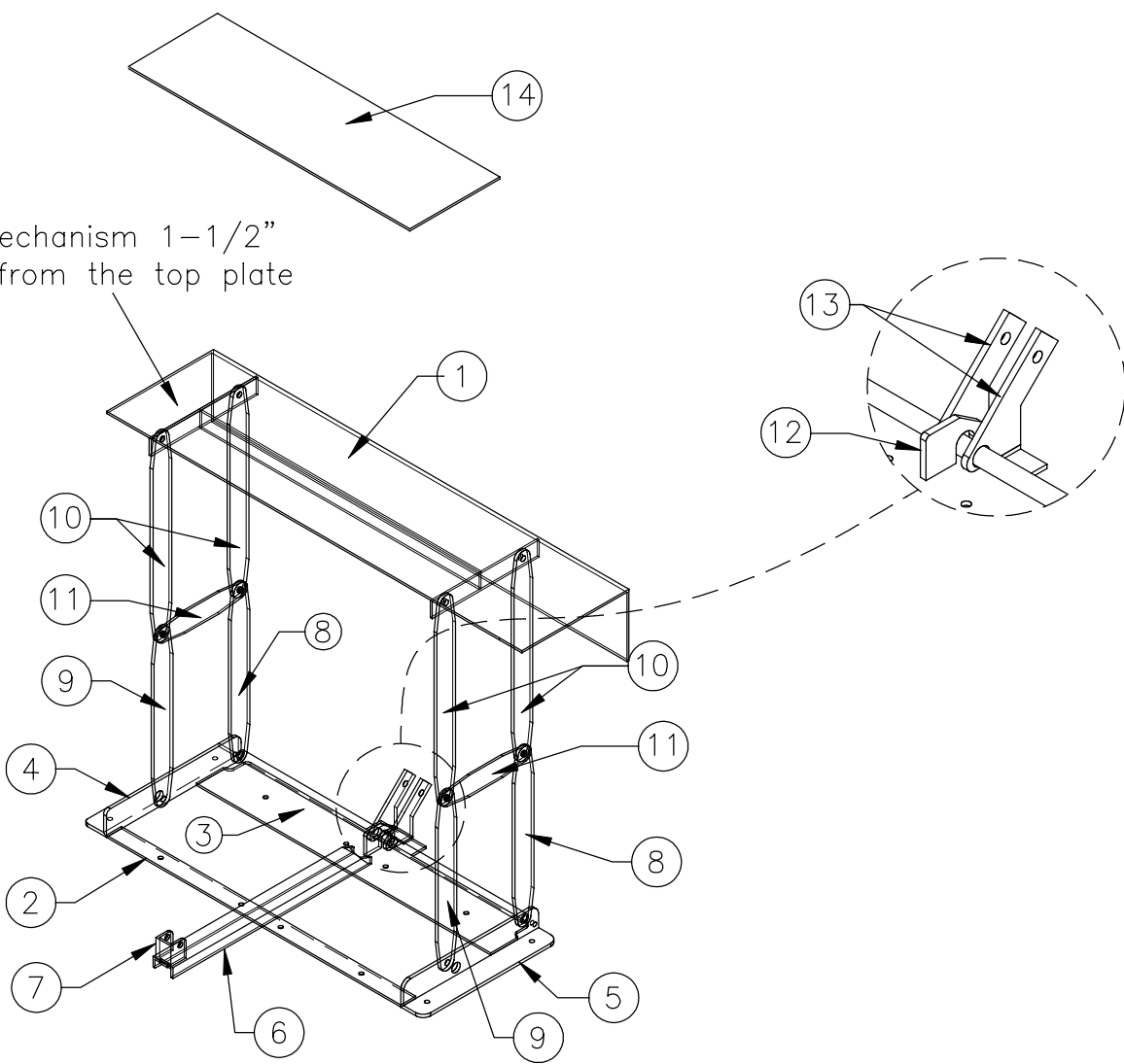
ISOMETRIC LAYOUT
