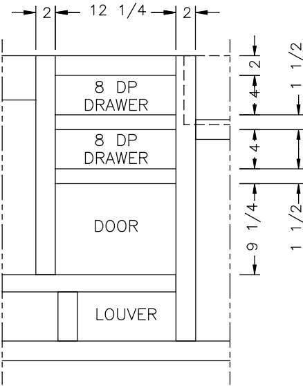
DRAWER SECTION DETAIL VIEW
