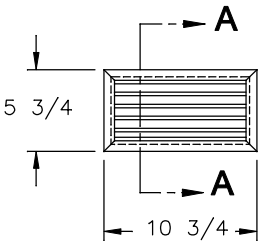
(2) 5 3/4 X 10 3/4 LOUVERED VENTS
