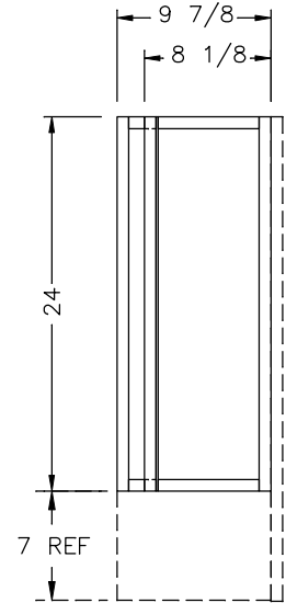
SECTION D
