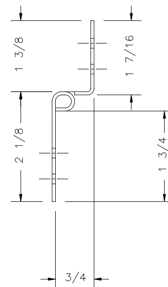
END VIEW
