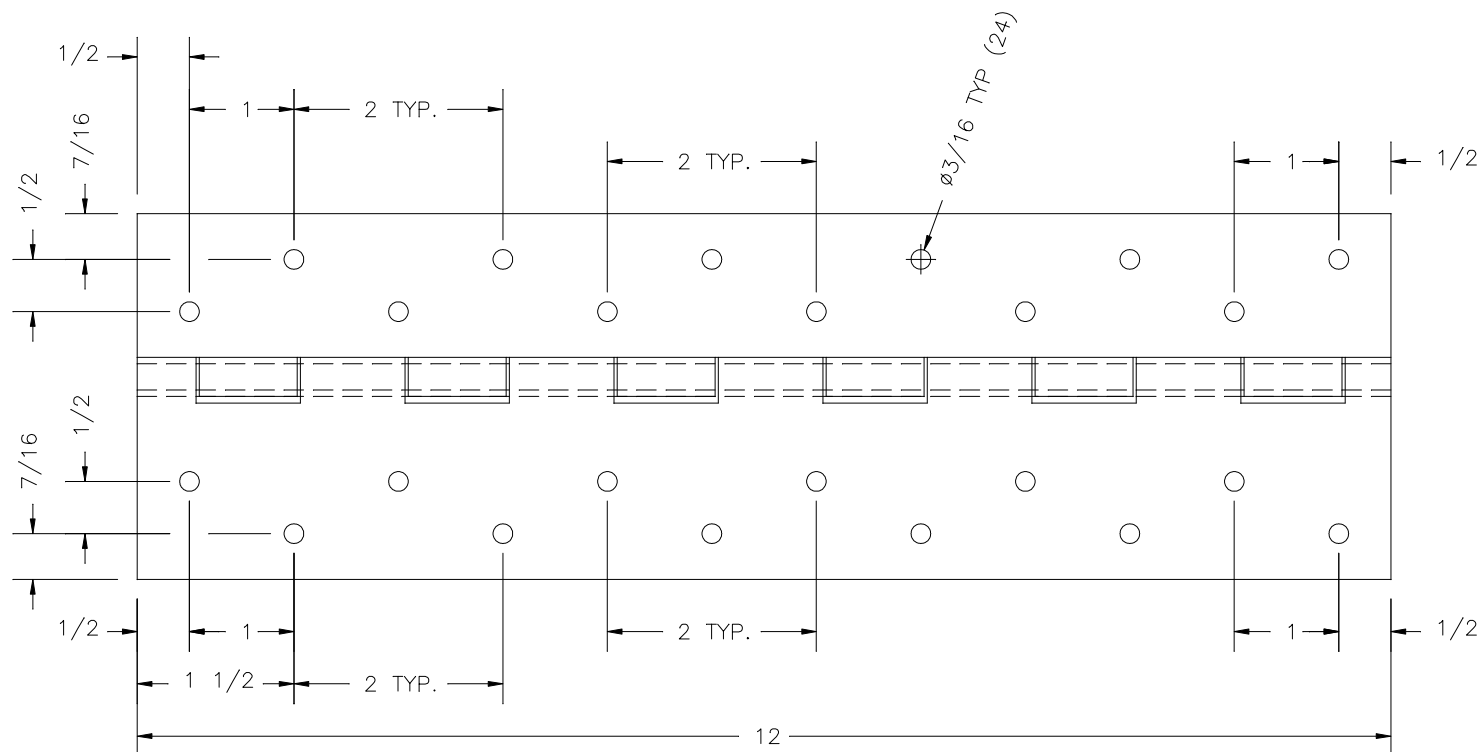
TOP VIEW
