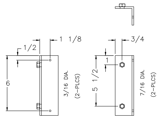
2x2x6 1/2x3/16 ANGLE
