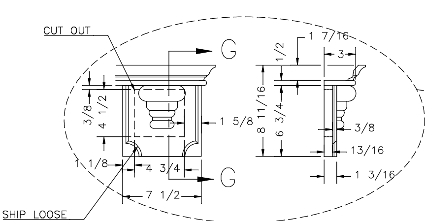
CAP BLOCK DETAIL SECTION G-G SCALE: X2
