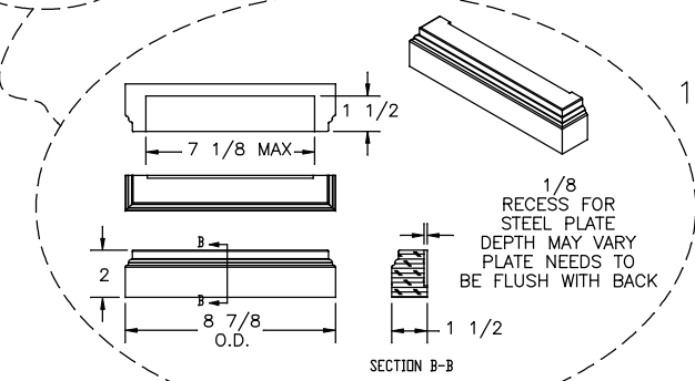
TOOL ACCESS BASE BOARD COVER DETAIL (REMOVABLE - ATTACHED WITH MAGNETS) SCALE: X2
