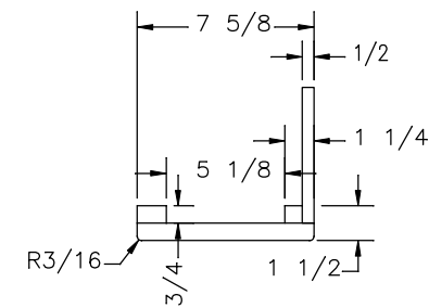
FOOT BLOCK CAP DETAIL SECTION B-B SCALE: X2
