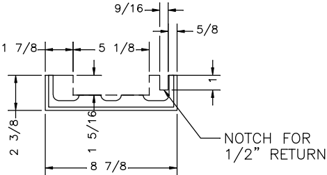
FOOT BLOCK CAP DETAIL SECTION E-E SCALE: X2
