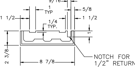
FOOT BLOCK CAP DETAIL SECTION F-F SCALE: X2
