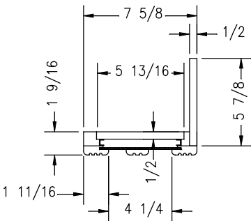
VERTICAL FASCIA DETAIL SECTION A-A SCALE: X4
