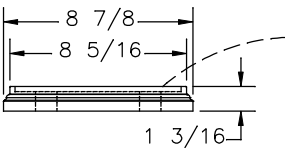
FOOT BLOCK CAP DETAIL SCALE: x2
