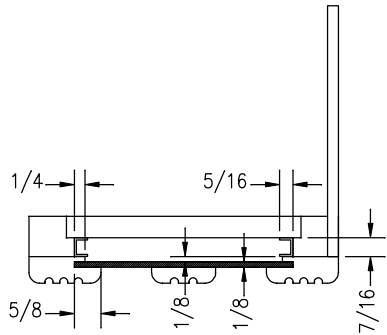
VERTICAL FASCIA DETAIL SECTION A-A SCALE: X4
