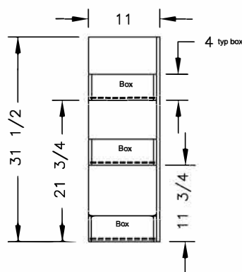
FRONT VIEW OF LEFT SIDE
