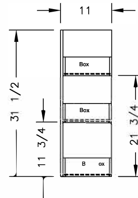
FRONT VIEW OF RIGHT SIDE
