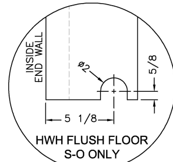
DETAIL D
