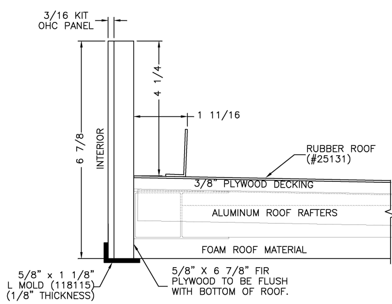
SECTION B-B KITCHEN
