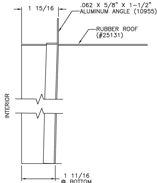
VIEW A BED BASE & WARDROBE SLIDEOUTS ONLY (MOTORIZED)
