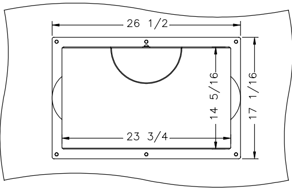
ASSEMBLED TOP VIEW WITHOUT LID/CUTTING BOARD
