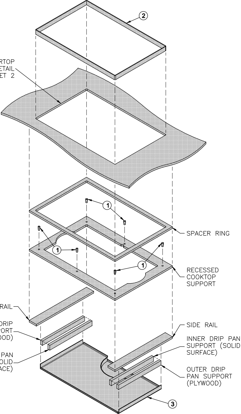
EXPLODED ISO VIEW (WITHOUT LID/CUTTING BOARD)
