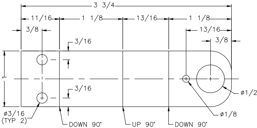
FLAT PATTERN VIEW
