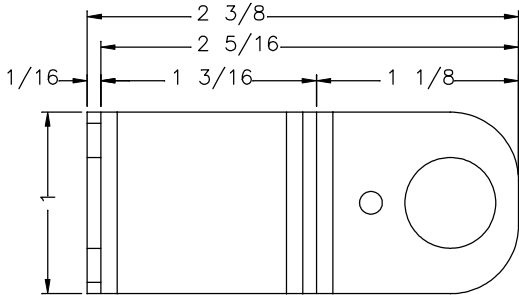
FRONT VIEW (BENT)
