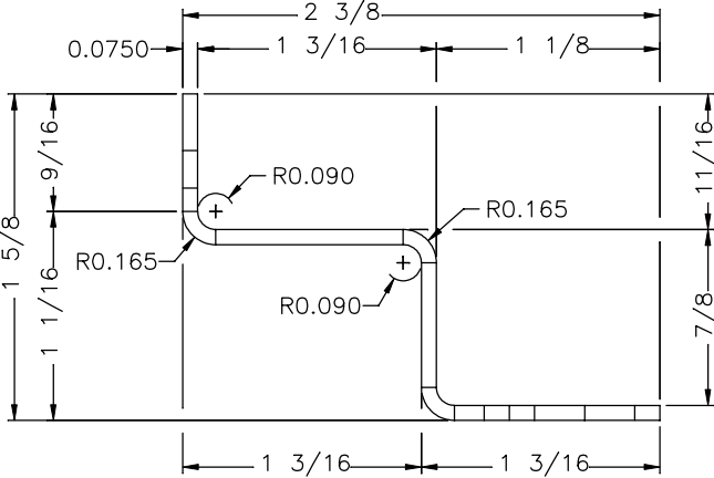
SIDE VIEW (BENT)
