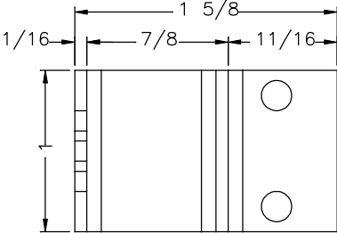
TOP VIEW (BENT)
