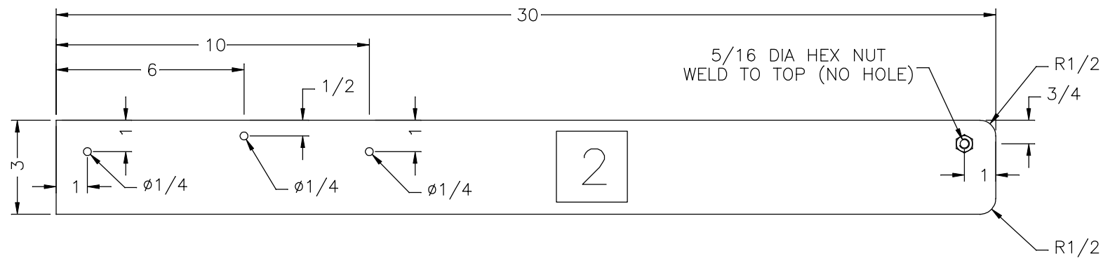
RIGHT BRACKET
