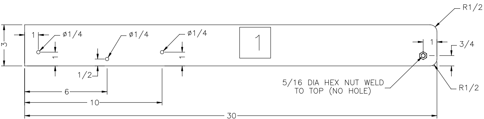
LEFT BRACKET
