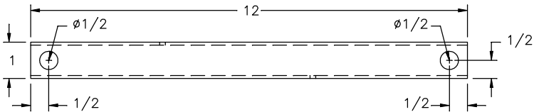
SWING ARM (TOP VIEW)
