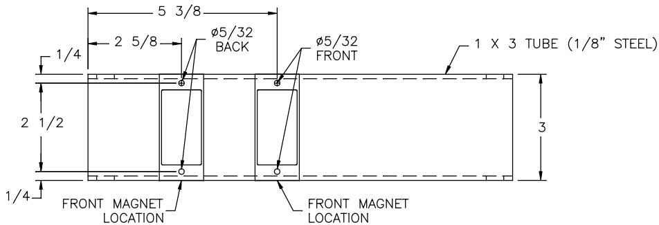
SWING ARM (FRONT VIEW)
