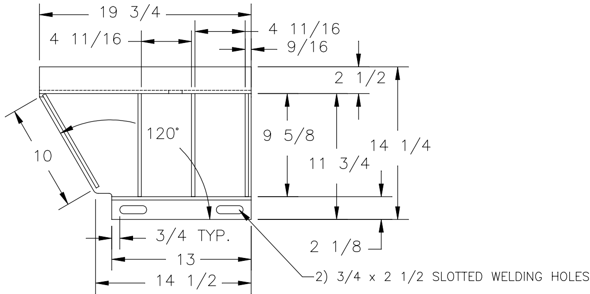
FRONT VIEW
